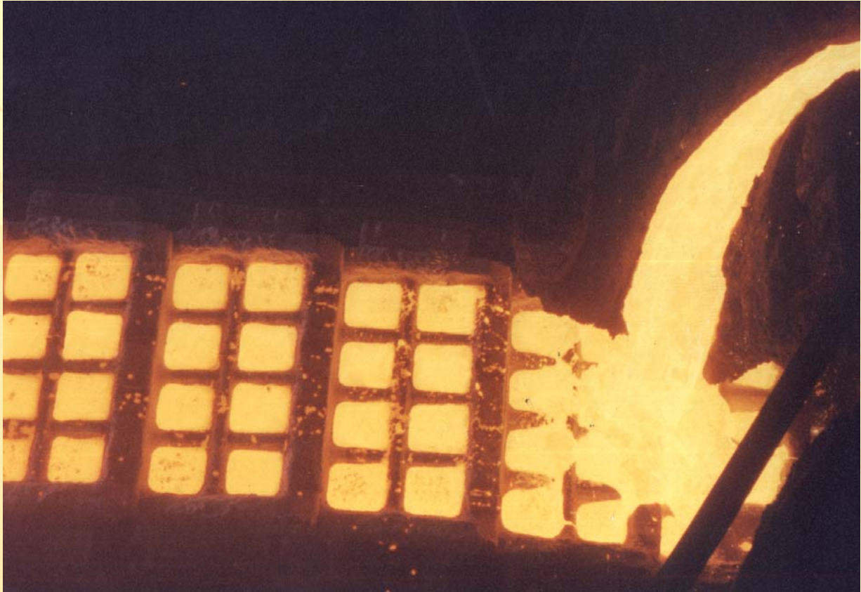
Continious Casting of Pig Iron in Our Mould
